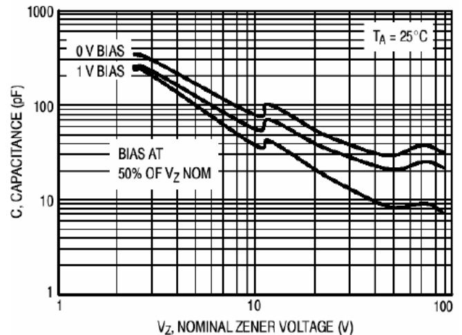
Fig 6. Typical Capacitance
