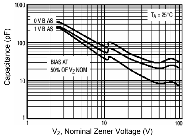
Figure 6. Typical Capacitance
