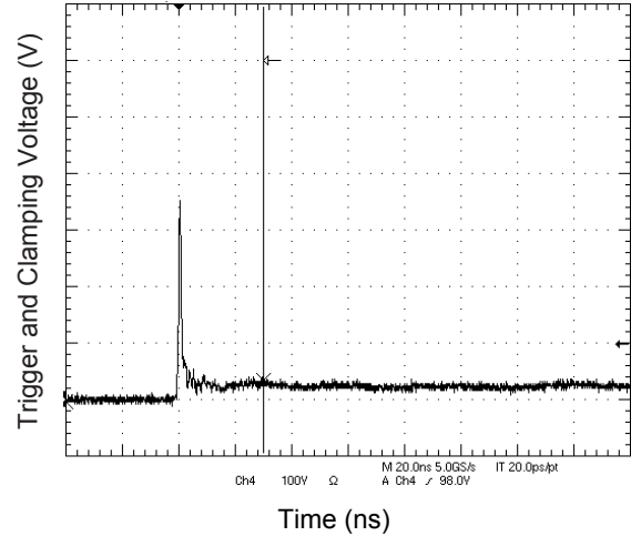
Figure 2. IEC61000-4-2 +8kV Contact Discharge
