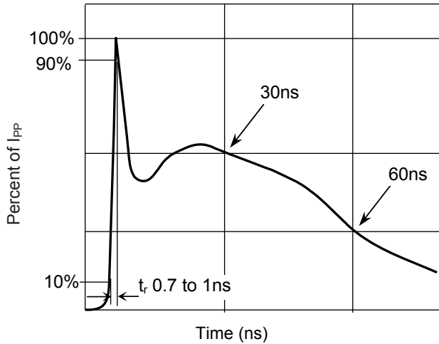
Figure 1. Pulse Waveform-ESD (IEC61000-4-2)
