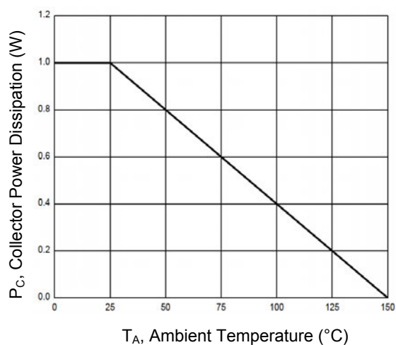
Figure 8. P_C - T_a
