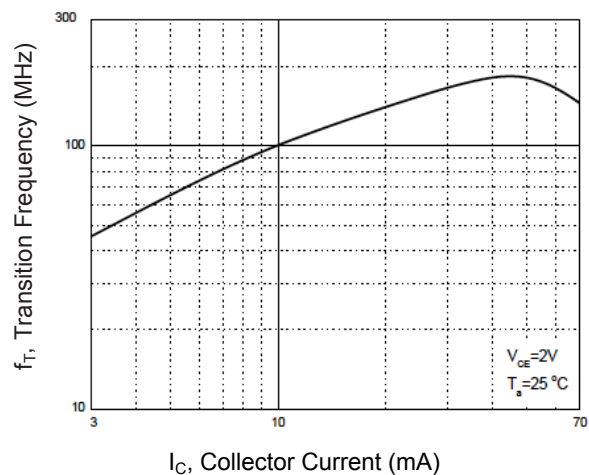
Figure 7. f_T - I_C
