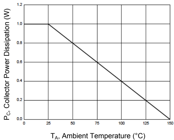
Figure 8. P_C - T_a
