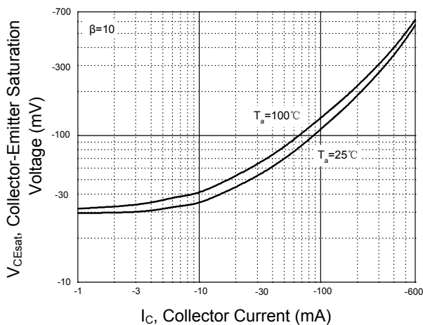
Figure 3. V_{CEsat} - I_C
