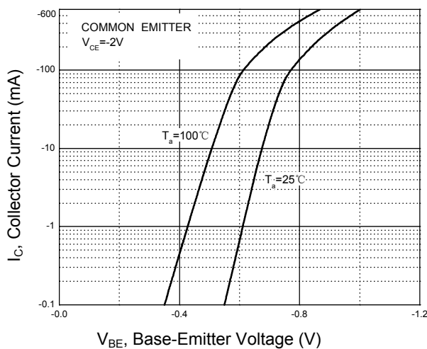
Figure 5. I_C - V_{BE}
