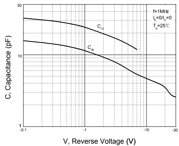
Figure 6. C_{ob}/C_{ib} - V_{CB}/V_{EB}
