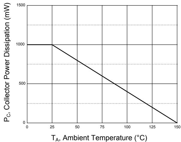
Figure 8. P_C - T_a
