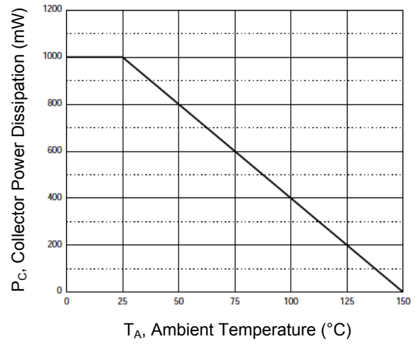
Figure 8. P_C - T_a
