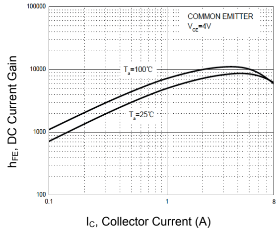
Figure 2. h_{FE} - I_C
