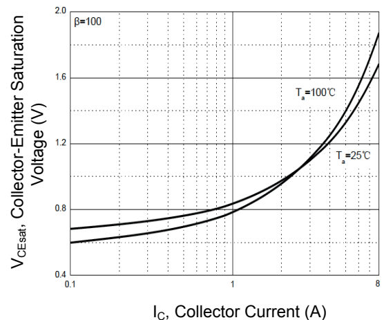
Figure 4. V_{CEsat} - I_C
