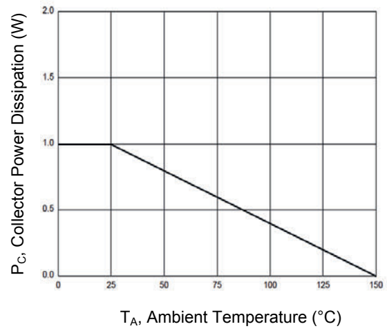
Figure 8. P_C — T_A
