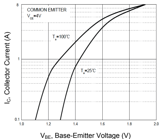
Figure 6. I_C - V_{BE}
