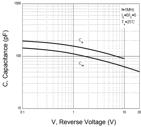
Figure 7. C_{ob}/C_{ib} — V_{CB}/V_{EB}
