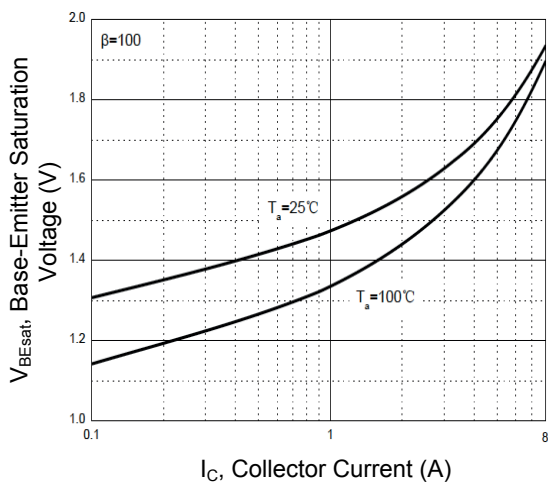
Figure 5. V_{BEsat} - I_C
