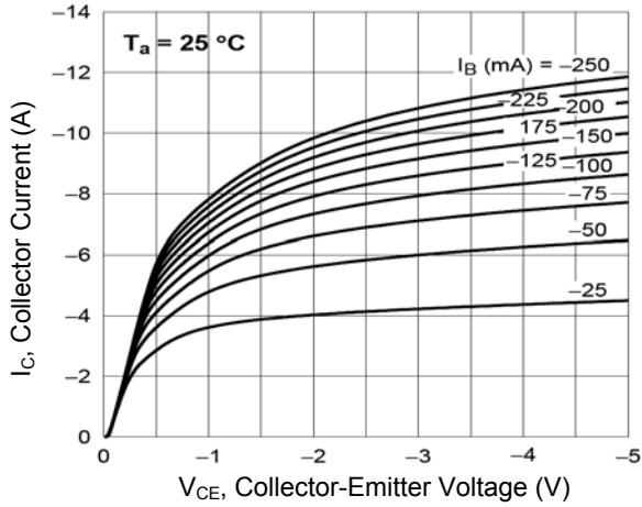
Figure 1. Static Characteristic
