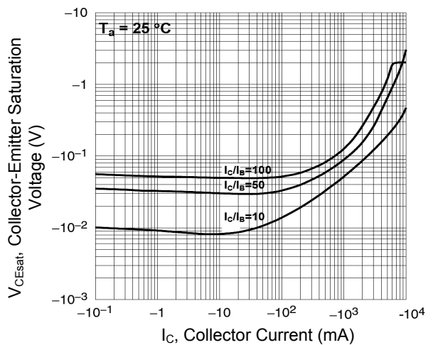
Figure 6. Collector-Emitter Saturation Voltage vs. Collector Current
