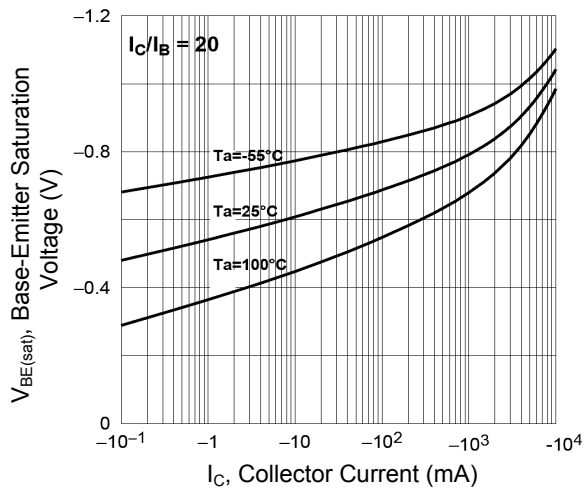
Figure 3. Base-Emitter Saturation Voltage vs. Collector Current
