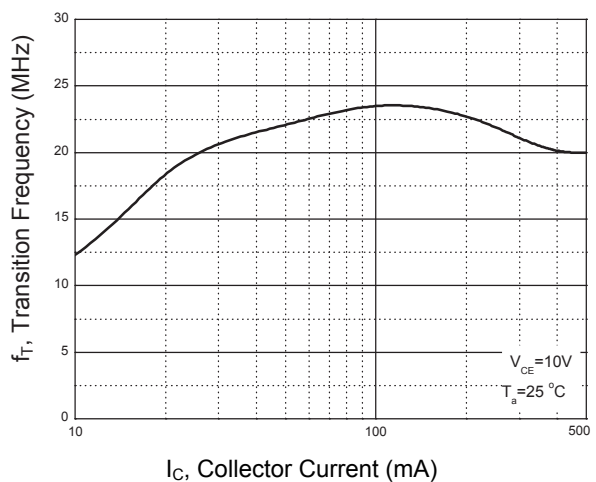
Figure 6. f_T - I_C
