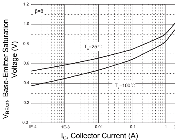
Figure 3. V_{BEsat} - I_C
