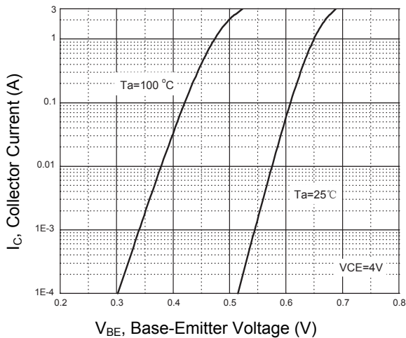
Figure 5. V_{BE} - I_C
