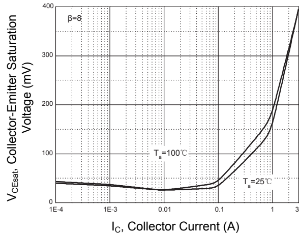
Figure 4. V_{CEsat} - I_C
