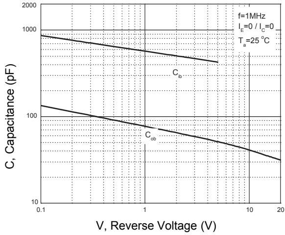
Figure 7. C_{ob}/C_{ib} - V_{CB}/V_{EB}
