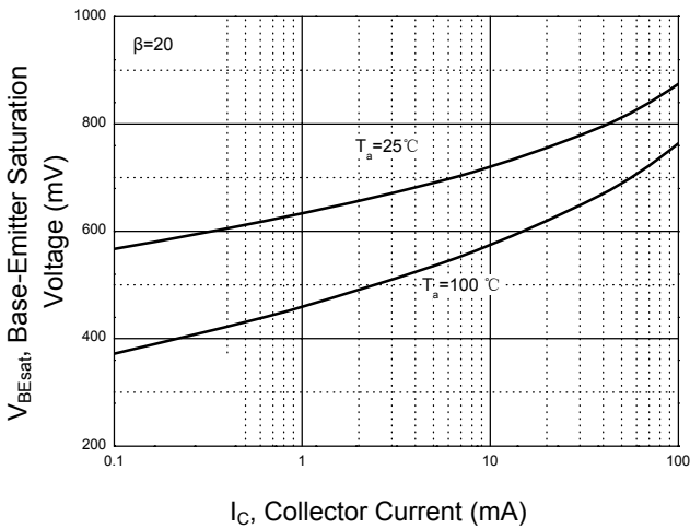
Figure 3. V_{BE(sat)} - I_C
