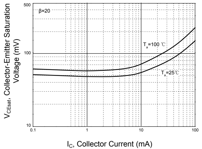
Figure 4. V_{CE(sat)} - I_C
