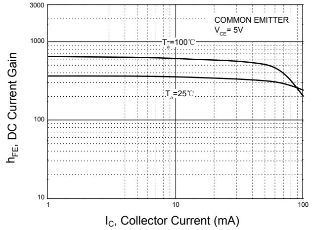
Figure 2. h_{FE} - I_C
