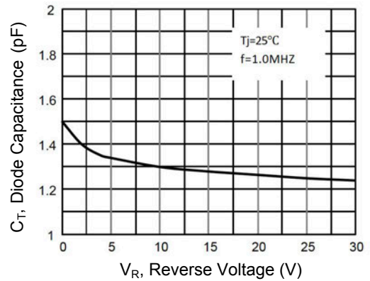
Figure 4. Capacitance Characteristics
