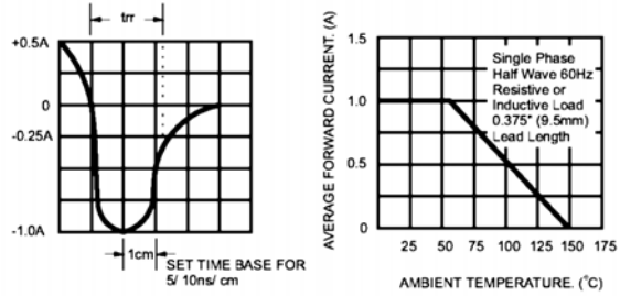
FIG. 2- MAXIMUM AVERAGE FORWARD CURRENT DERATING
