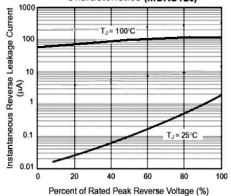
Fig. 4 – Typical Reverse Leakage Characteristics (MURS120)
