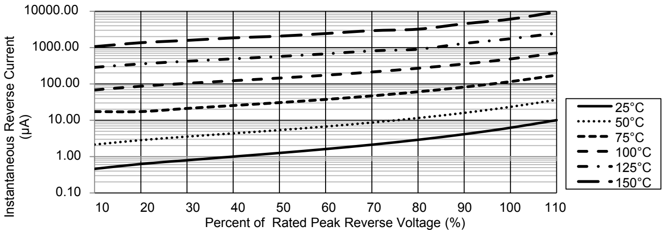
Figure 4. Typical Reverse Characteristics (SK12 thru SK14)
