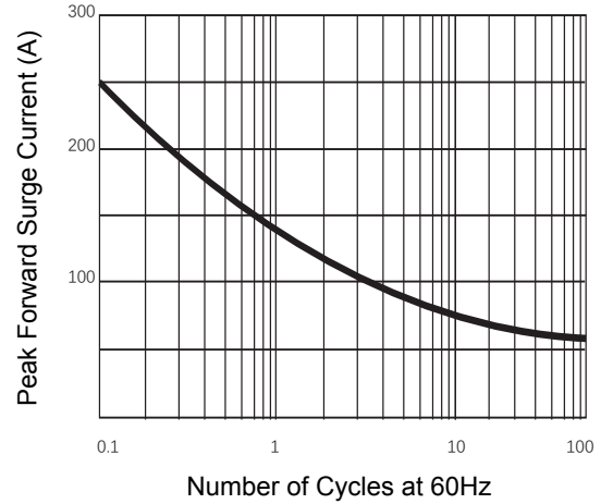
Figure 2. Max. Non-Repetitive Peak Forward Surge Current
