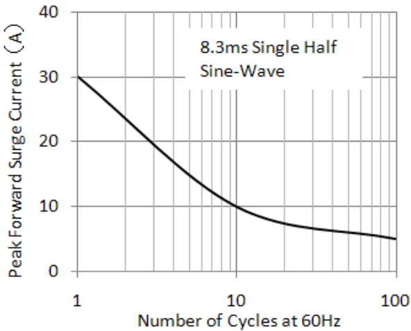
Figure 5. Maximum Non-Repetitive Peak Forward Surge Current
