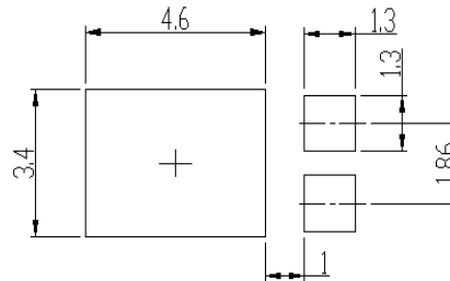
Soldering footprint
