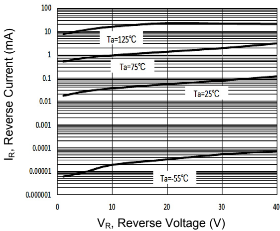
Figure 3. Reverse Characteristic Curve
