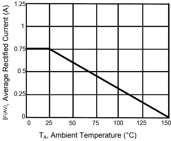
Figure 1. Average Rectified Current Derating Curve
