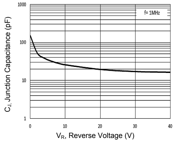
Figure 4. Junction Capacitance
