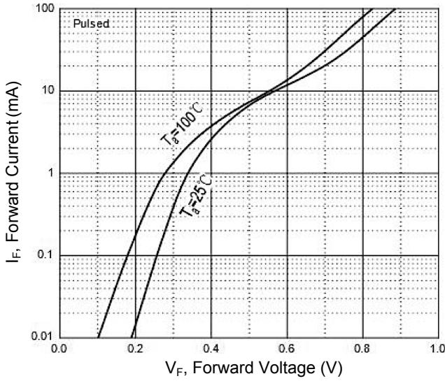
Figure 1. Forward Characteristics
