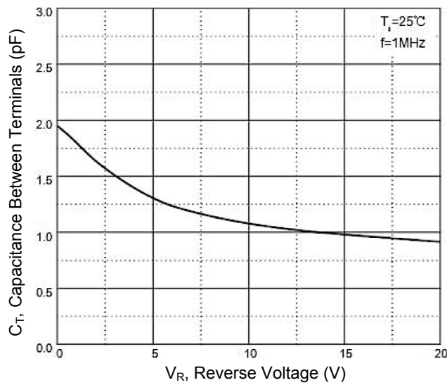
Figure 3. Capacitance Characteristics
