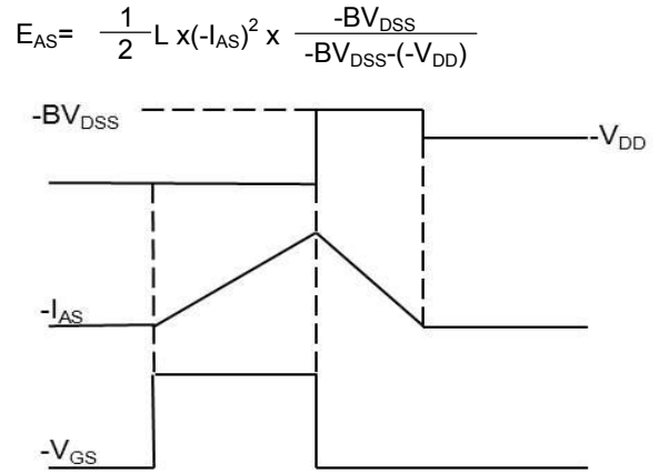
Figure 8. EAS Waveform
