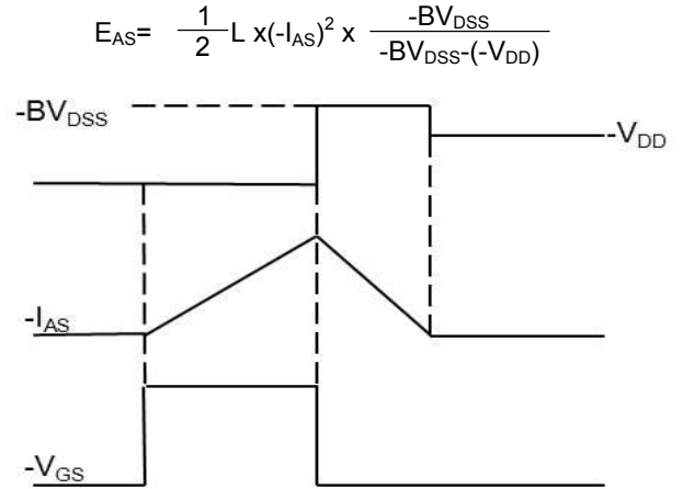
Fig.8 E_{AS} Waveform
