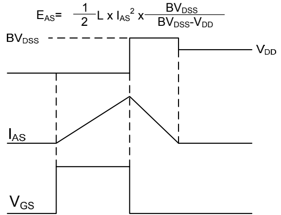
Fig.8 E_{AS} Waveform
