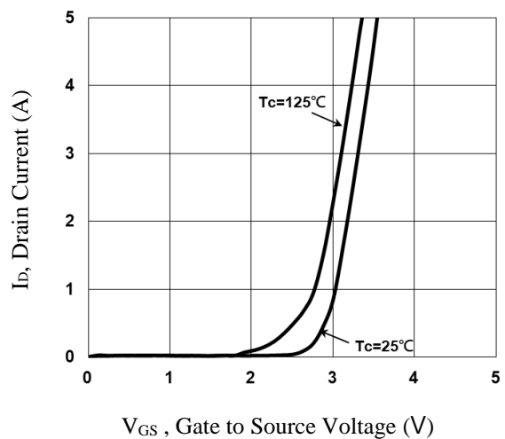
Fig.6 Transfer Characteristics
