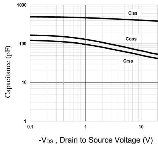
Fig.6 Capacitance Characteristics
