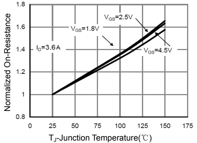
Figure 8 Drain-Source On-Resistance
