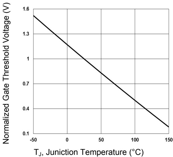
Fig.3 Normalized Gate Threshold Voltage vs. T J
