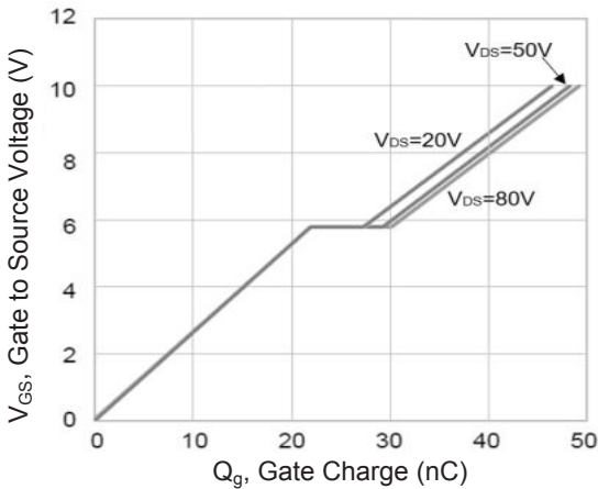
Figure 3. Gate Charge
