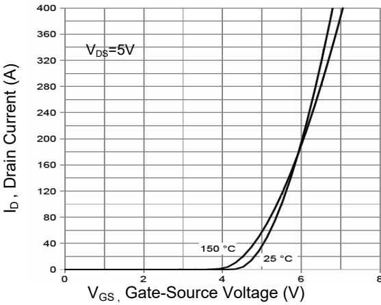
Figure 3. Transfer Characteristics
