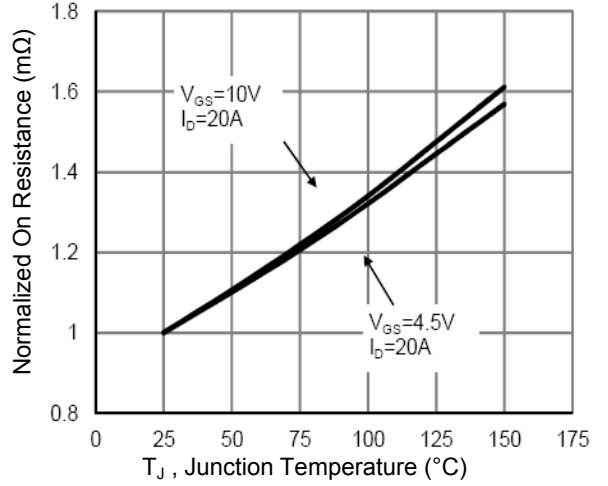
Figure 2. Rdson-Junction Temperature
