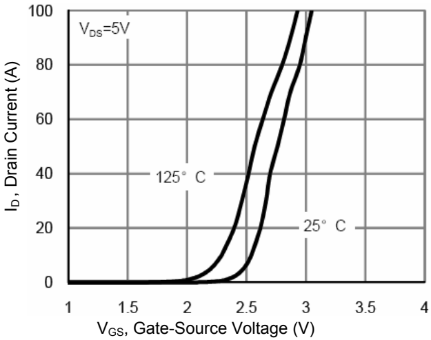
Figure 3. Transfer Characteristics
