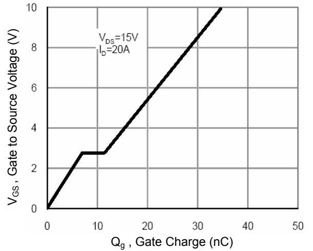
Figure 4. Gate Charge
