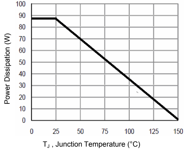
Figure 8. Power De-Rating
