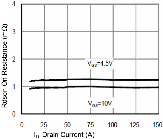
Figure 5. R_{DS(ON)} -Drain Current
