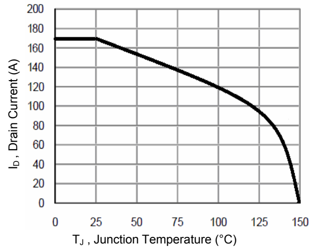
Figure 10. Current De-Rating
