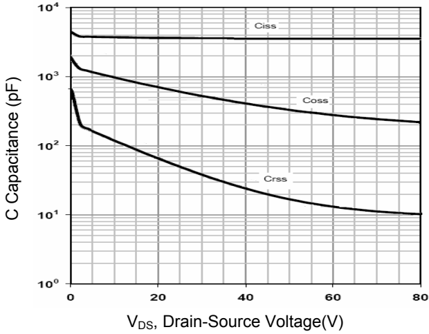
Figure 7. Capacitance Characteristics
