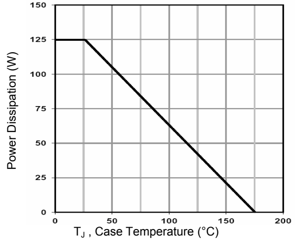
Figure 8. Power De-rating
