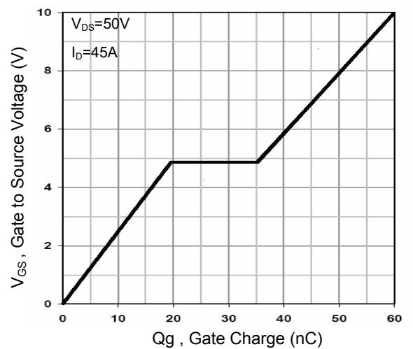
Figure 4. Gate Charge
