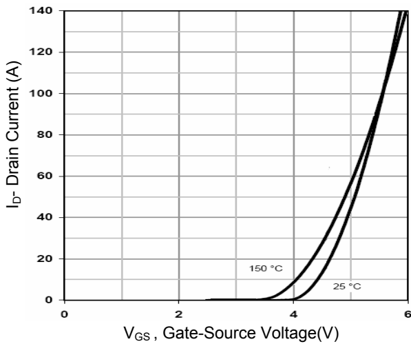
Figure 3. Transfer Characteristics
