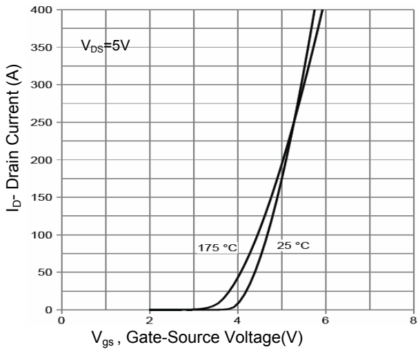
Figure 3. Transfer Characteristics
