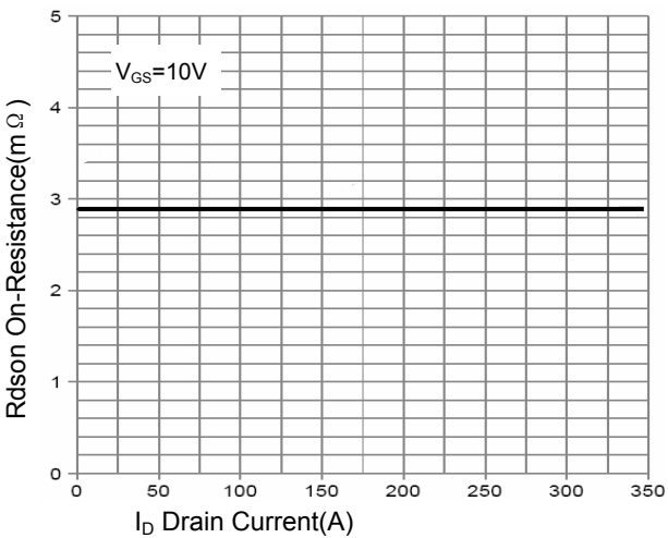
Figure 5. Rdson-Drain Current
