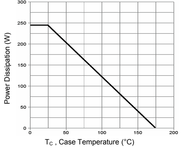
Figure 8. Power De-rating
