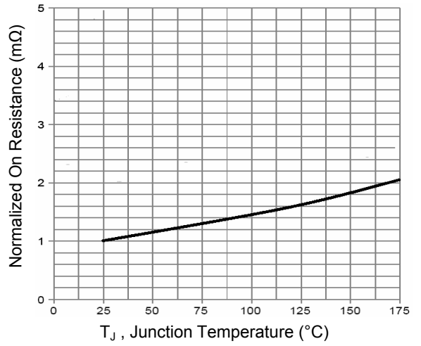
Figure 2. Rdson-Junction Temperature
