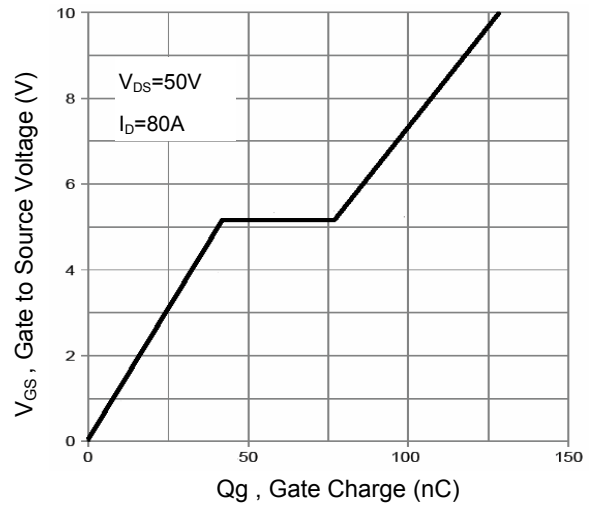
Figure 4. Gate Charge
