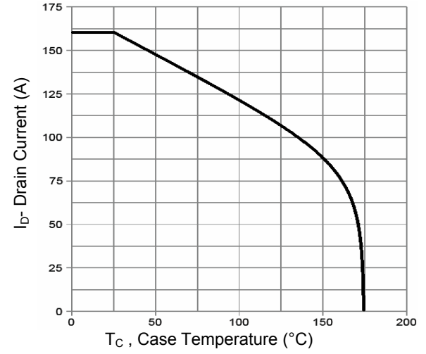
Figure 10. Current De-rating
