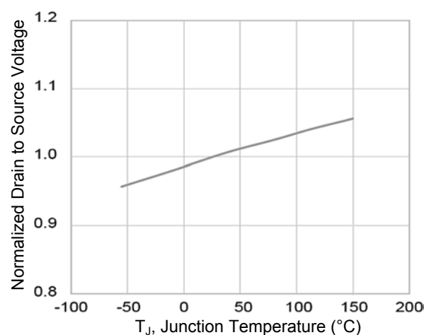
Figure 6. Normalized BV_{DSS} vs. T_J
