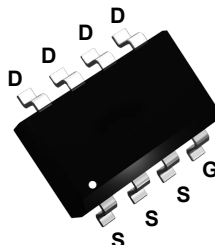
SOP-8
