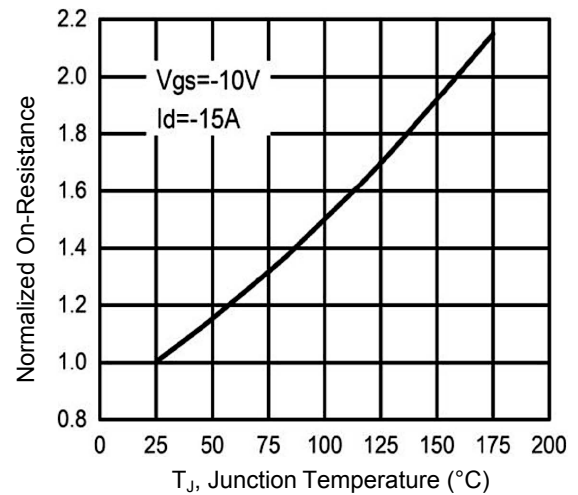
Figure 4. Normalized On-Resistance vs. T_J
