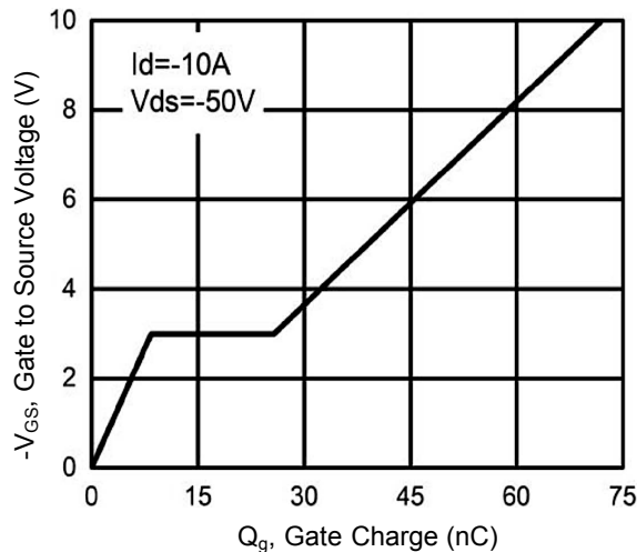
Figure 3. Gate Charge
