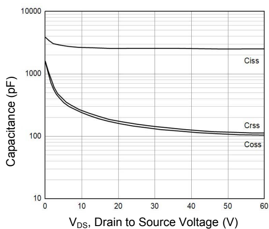
Figure 4. Capacitance Characteristics
