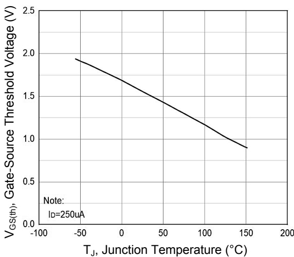
Figure 5. V_{GS(th)} vs. T_J
