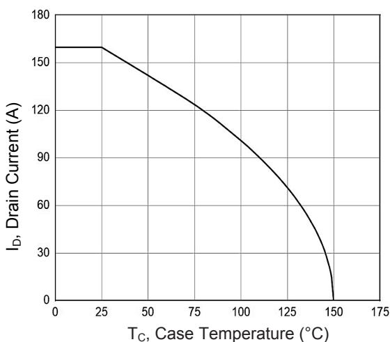
Figure 12. Drain Current vs. T_C
