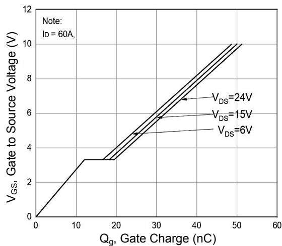
Figure 8. Gate Charge vs. V_{GS}
