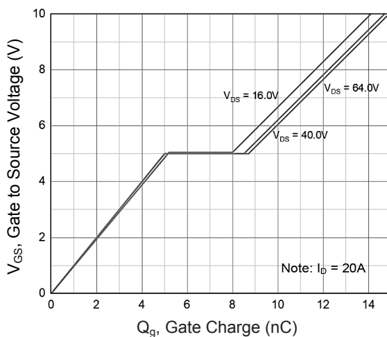
Figure 3. Gate Charge
