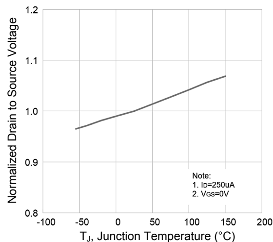
Figure 6. Normalized BV_{DS(sat)} vs. T_J
