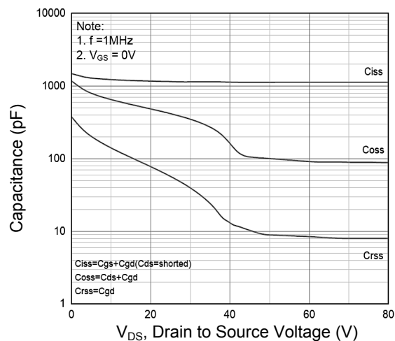
Figure 8. Capacitance Characteristics
