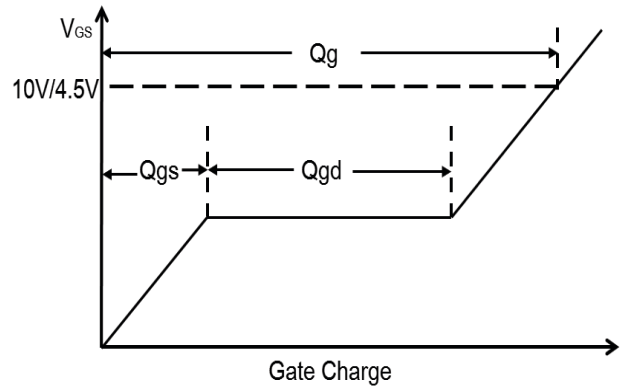
Figure 11. Gate Charge Waveform
