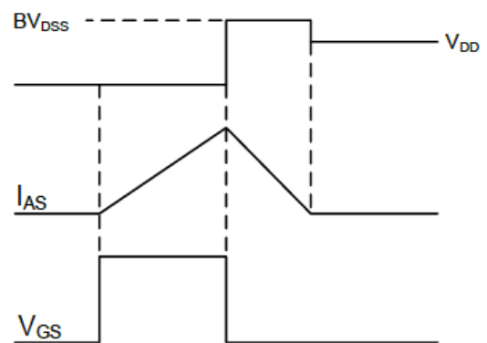
Figure 12. EAS Waveform
