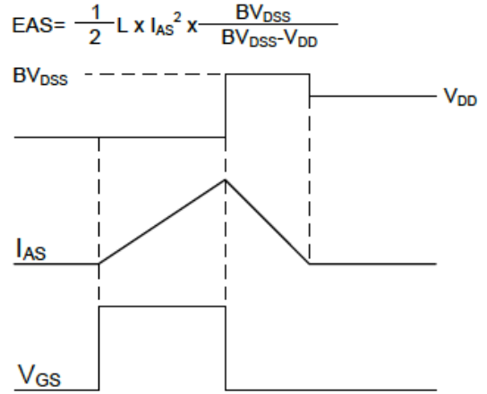
Figure 8. EAS Waveform
