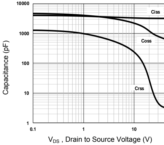
Figure 7. Capacitance Characteristics
