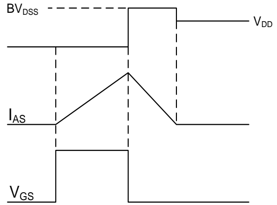
Figure 8. EAS Waveform
