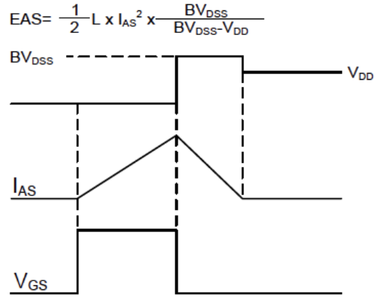
Figure 8. EAS Waveform
