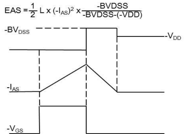
Fig.10 EAS Waveform
