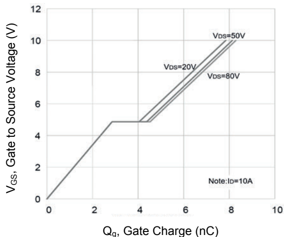
Figure 6. Gate Charge
