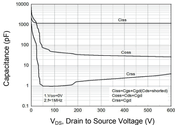
Figure 7. Capacitance Characteristic
