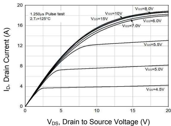
Figure 2. Transfer Output Characteristics
