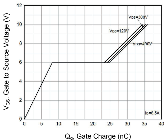
Figure 6. Gate Charge Characteristic
