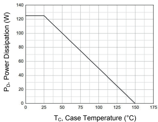
Figure 13. Power Dissipation vs. T_C
