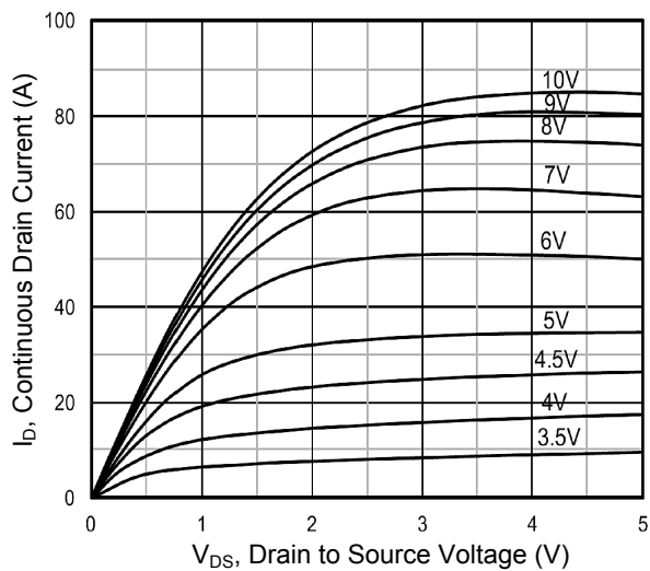
Figure 1. Output Characteristics Curve
