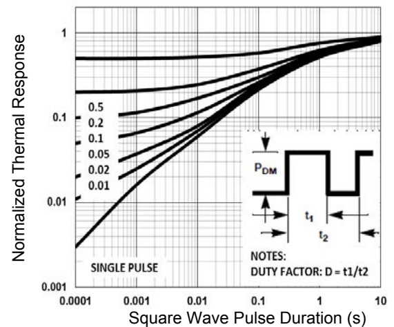
Figure 6. Normalized Transient Impedance
