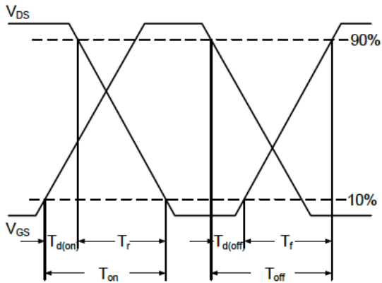
Figure 8. Switching Time Waveform
