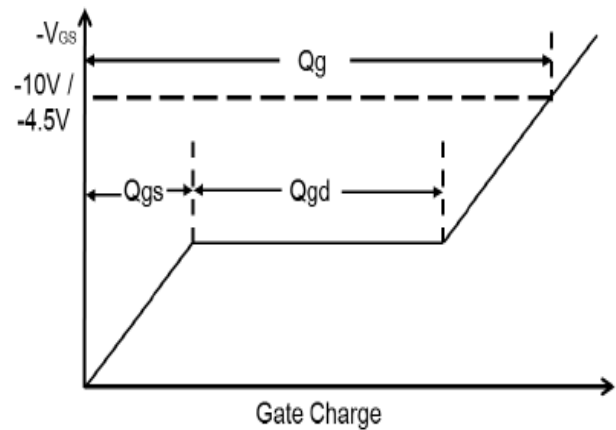
Figure 10. Gate Charge Waveform
