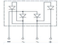
Schematic Diagram
